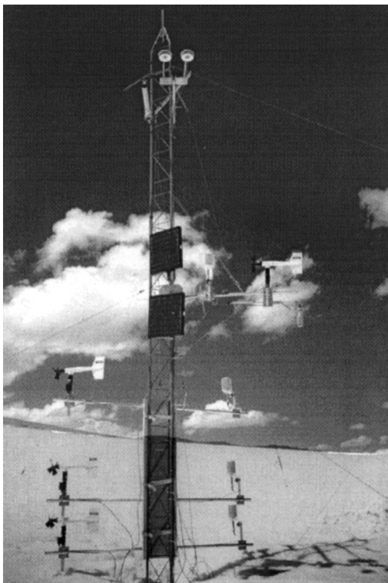
Figure 2. The meteorological tower at the subnivean laboratory on Niwot Ridge. Temperature, relative humidity and wind speed are collected at 0.5, 1.0 and 2.0 meters above the snowpack to calculate latent heat fluxes via the aerodynamic profile method. Instrumentation is mounted on a fixed mast which can be adjusted according to snow height
