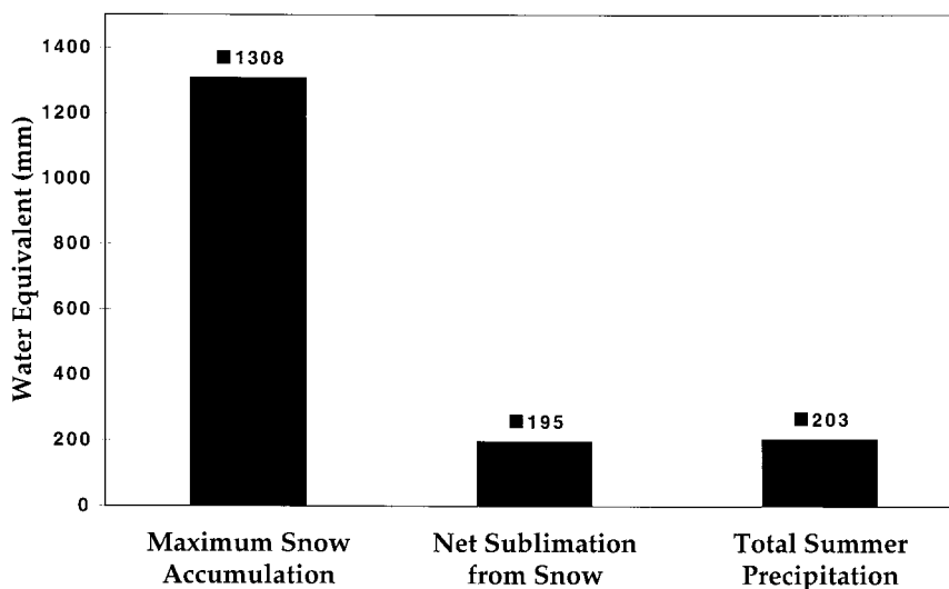
Figure 5. Mass loss from the snowpack in the context of other precipitation totals. Sublimation from the seasonal snowpack is an important component of the alpine hydrologic cycle. The 195 mm of water equivalent lost to sublimation was greater than 15% of the maximum snow accumulation and nearly equivalent to the total precipitation for the entire summer season
