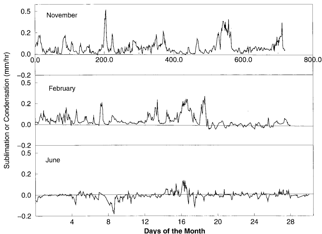
Figure 6. Hourly moisture fluxes between the snowpack and atmosphere for November, February and June. Positive fluxes indicate sublimation while negative fluxes indicate condensation. November and February are dominated by sublimation, whereas June features both sublimation and condensation as well as significantly lower moisture flux rates
