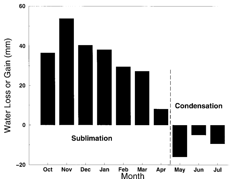
Figure 4. Monthly net sublimation and condensation for the 1994–1995 snow season. Most of the sublimation occurs during the snow accumulation season. During snowmelt season in the early summer, there is net condensation from the atmosphere to the snowpack
