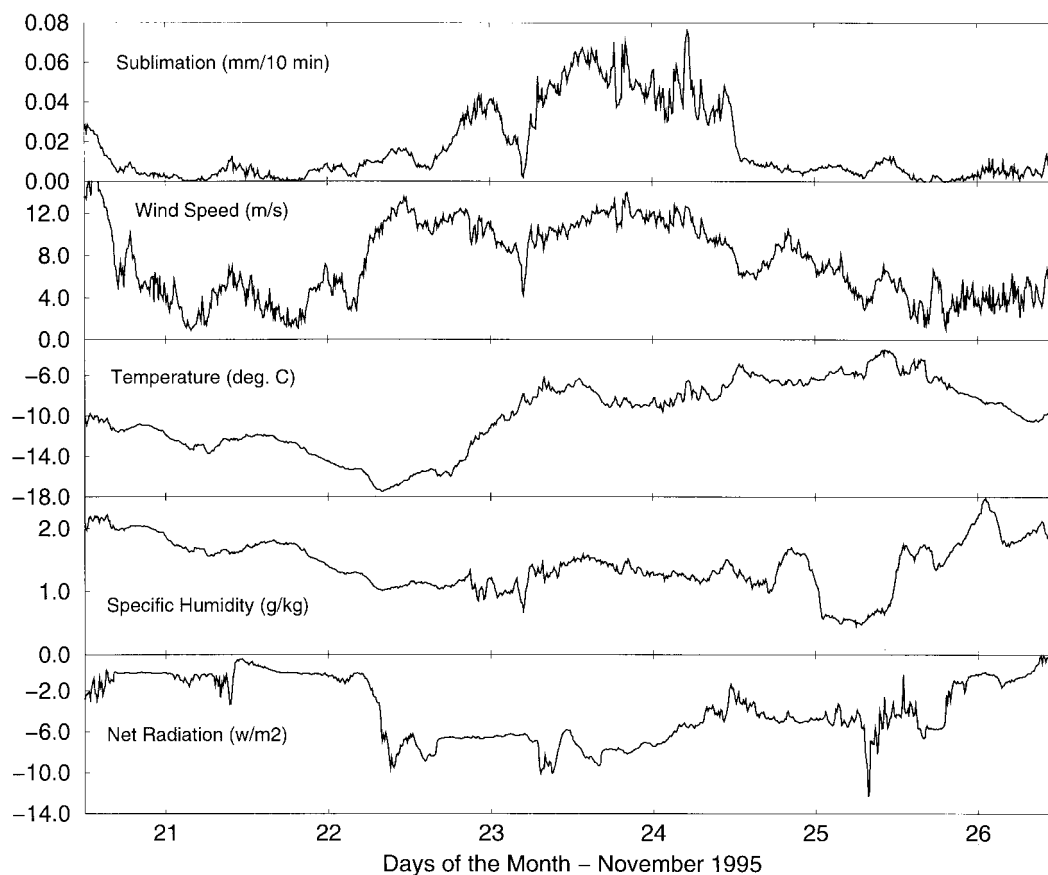
Figure 7. Times series of ten-minute averages for sublimation, wind speed, temperature, specific humidity, and net radiation during six days in November. Tick marks denote the beginning of each day. All measurements were taken from the 1.0 m height in the instrument profile except net radiation which was measured at 6.0 m. Sublimation was most closely correlated with wind speed ( r^2 = 0.56 , p \ll 0.001 , n = 865 ), particularly during the sublimation event on 22–24 November ( r^2 = 0.66 , p \ll 0.001 , n = 239 )
