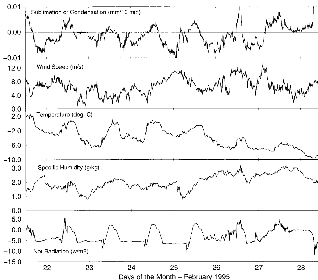
Figure 8. Times series of ten-minute averages for sublimation, wind speed, temperature, specific humidity, and net radiation during seven days in February. Tick marks denote the beginning of each day. All measurements were taken from the 1.0 m height in the instrument profile except net radiation which was measured at 6.0 m. Moisture fluxes were most closely correlated with net radiation ( r^2 = 0.32 , p \ll 0.001 , n = 1009 ). During the first five days of this period, temperature also showed a moderate correlation with the moisture flux ( r^2 = 0.29 , p \ll 0.001 , n = 648 )
